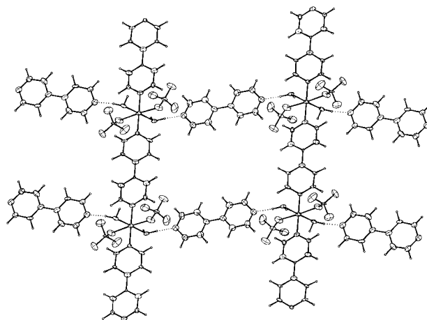
Fig. 1 Two-dimensional architecture 11 of the structure of [Cu( \mu -4,4'-bipy)(H 2 O) 2 (FBF 3 ) 2 ] \cdot 4,4'-bipy, showing the Cu–4,4'-bipy–Cu (co-ordinated) and Cu–OH 2 \cdots 4,4'-bipy \cdots H 2 O–Cu (hydrogen bonded) 4,4'-bipy bridges
