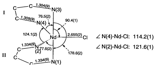
Fig. 3 Molecular structure and atom numbering scheme for [\text{Nd}(\text{L-L})_2\text{Cl}] \mathbf{5}
