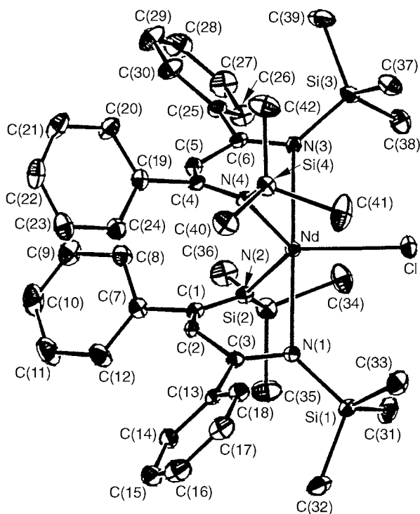
Fig. 3 Molecular structure and atom numbering scheme for [\text{Nd}(\text{L-L})_2\text{Cl}] \mathbf{5}
