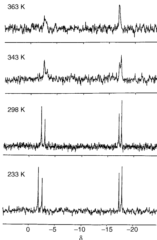
Fig. 2 Variable-temperature ^{29}\text{Si} - \{^1\text{H}\} NMR spectra of [\text{Yb}(\text{L-L}')_2] 13 (49.7 MHz, in \text{C}_6\text{D}_5\text{CD}_3 )
