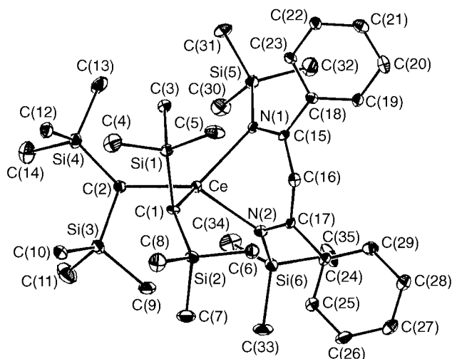
Fig. 5 Molecular structure and atom numbering scheme for [\text{Ce}(\text{L-L})(\text{CHR}_2)_2] \mathbf{9}
