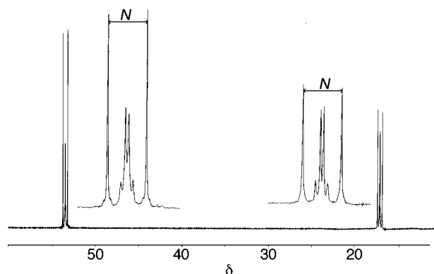
Fig. 4 The 31 P- 1 H NMR spectrum (101.25 MHz) of complex 4a , formed in situ by treating a deuteriochloroform solution of 2a with 2 mol equivalents of CF 3 CO 2 H. The spectrum is of the AA'XX' type and deceptively simple. The doublet of separations N = |J(P_F P_S) + J(P_S P_S)| are shown
