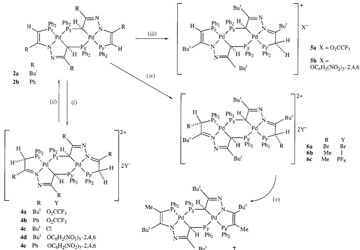
Scheme 3 (i) At least 2 mol equivalents of CF 3 CO 2 H, HCl or 2,4,6-(O 2 N) 3 C 6 H 2 OH; (ii) NaOMe; (iii) 1 equivalent of CF 3 CO 2 H; (iv) Br 2 -CCl 4 or MeI, with NH 4 PF 6 added for 6c ; (v) KOBu t
