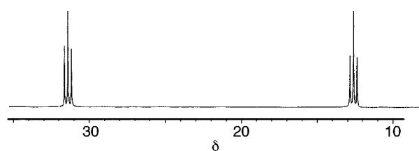
Fig. 1 The ^{31}\text{P}\{-^1\text{H}\} NMR spectrum (101.25 MHz) of complex 2a in deuteriochloroform showing the 'deceptively simple' triplets of the AA'XX' spin system with N = |J(\text{P}_F\text{P}_S) + J(\text{P}_F\text{P}_S)| = 46 Hz
