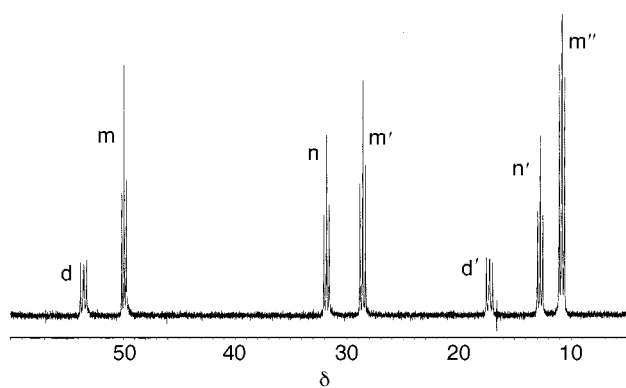
Fig. 5 The 31 P-{ 1 H} NMR spectrum (101.25 MHz) of the mixture of complexes 2a , 4a and 5a , formed by treating 2a with 1 mol equivalent of CF 3 CO 2 H. The resonances are identified as follows: n and n' for the neutral complex 2a , m, m' and m'' for the monoprotonated complex 5a and d and d' for the diprotonated complex 4a ; the linkages were established by a 31 P- 31 P COSY experiment. The chemical shifts of the phosphorus atoms of 5a with the separation of the outer peaks of the three 'deceptively simple' patterns are as follows: m, δ 49.9(t), separation 42.5 Hz; m' δ 28.6(t), separation 49.5 Hz; m'', δ ≈ 10.9(q), separation 46 Hz
