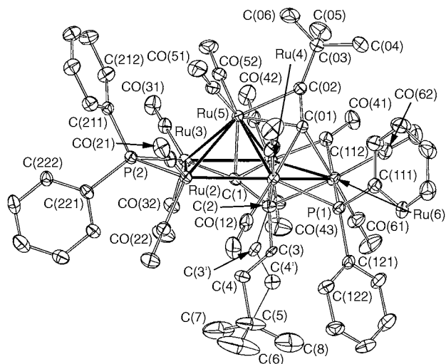
Fig. 2 Plot of a molecule of [\text{Ru}_6(\mu_6\text{-C}_2\text{CH=CHBu}^t)(\mu_3\text{-C}_2\text{Bu}^t)(\mu\text{-PPh}_2)_2(\mu\text{-CO})(\text{CO})_{12}] 3 showing the atom numbering scheme. Significant bond lengths (Å) and angles ( ^\circ ): Ru(1)–Ru(2) 2.890(1), Ru(1)···Ru(4) 3.880(2), Ru(1)–Ru(5) 2.8468(7), Ru(1)–Ru(6) 2.779(3), Ru(2)–Ru(3) 2.775(2), Ru(2)–Ru(5) 2.786(2), Ru(3)–Ru(4) 2.798(2), Ru(4)–Ru(5) 2.848(2), Ru(4)–Ru(6) 2.8053(9), Ru(1)–P(1) 2.329(2), Ru(6)–P(1) 2.312(2), Ru(2)–P(2) 2.275(2), Ru(3)–P(2) 2.291(3), Ru(1)–C(1) 2.413(6), Ru(2)–C(1) 2.136(6), Ru(3)–C(1) 2.127(6), Ru(4)–C(1) 2.204(6), Ru(5)–C(1) 2.100(6), Ru(1)–C(2) 2.340(6), Ru(4)–C(2) 2.238(6), Ru(6)–C(2) 2.260(6), Ru(1)–C(01) 2.168(6), Ru(5)–C(01), 2.211(6), Ru(6)–C(01), 2.210(6), Ru(5)–C(02) 2.269(6), C(1)–C(2) 1.426(8), C(01)–C(02) 1.245(8); Ru(1)–P(1)–Ru(6) 73.58(8), Ru(2)–P(2)–Ru(3) 74.83(5), C(01)–C(02)–C(03) 155.4(6)
