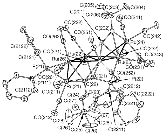
Fig. 1 Plot of molecule 2 of [\text{Ru}_6(\mu_3\text{-Bu}^t\text{CH}=\text{CHC}_2\text{PPh}_2)(\mu_4\text{-C}_2\text{Bu}^t)(\mu\text{-PPh}_2)(\text{CO})_{13}] 2 showing the atom numbering scheme. In this and subsequent figures, non-hydrogen atoms are shown with 20% thermal envelopes; hydrogen atoms have arbitrary radii of 0.1 Å. Significant bond lengths (Å) and angles (°) (for molecule 1 ): Ru(1)–Ru(2) 2.815(1), Ru(1)–Ru(6) 2.6952(9), Ru(2)–Ru(3) 2.820(1), Ru(2)–Ru(5) 2.6693(9), Ru(2)–Ru(6) 2.865(1), Ru(3)–Ru(4) 2.759(1), Ru(3)–Ru(5) 2.829(1), Ru(4)–Ru(5) 2.905(2), Ru(1)–P(1) 2.252(2), Ru(6)–P(1) 2.299(2), Ru(3)–P(2) 2.308(2), Ru(1)–C(2) 2.241(6), Ru(6)–C(2) 2.202(7), Ru(2)–C(1) 2.149(6), Ru(5)–C(1) 2.315(6), Ru(2)–C(01) 2.019(6), Ru(3)–C(01) 2.093(7), Ru(5)–C(01) 2.105(7), Ru(3)–C(02) 2.465(7), Ru(4)–C(02) 2.077(6), C(1)–C(2) 1.44(1), C(01)–C(02) 1.37(1), C(2)–C(3) 1.49(1), C(3)–C(4) 1.28(1), C(4)–C(5) 1.51(1); Ru(1)–P(1)–Ru(6) 72.62(7), Ru(3)–P(2)–C(1) 93.5(2), P(2)–C(1)–C(2) 139.4(5), C(2)–C(3)–C(4) 127.1(8), C(3)–C(4)–C(5) 131.3(9), C(01)–C(02)–C(03) 130.0(6)
