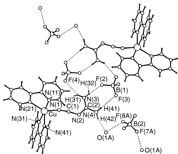
Fig. 3 Hydrogen-bonding interactions within the crystal structure of [Cu(bipy) 2 (cnge)][BF 4 ] 2 ·H 2 O 5
