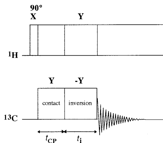
Fig. 4 An IRCP sequence based on a standard 13 C CP MAS experiment: 48 t_{\text{CP}} = contact time (fixed) and t_i = inversion time (variable)
