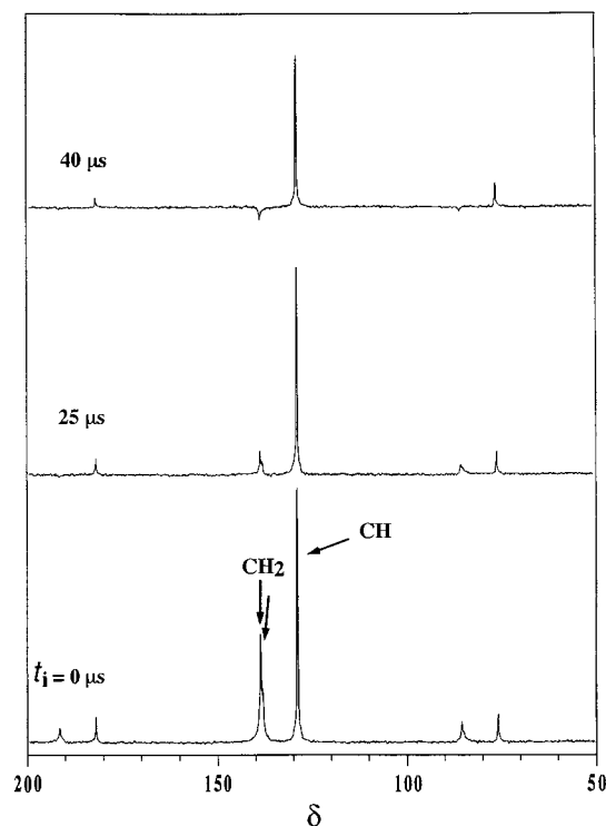
Fig. 5 The ^{13}\text{C} IRCP MAS NMR spectra of compound 1 ( t_{CP} = 5 ms); t_i = 0 \mu\text{s} corresponds to a standard CP MAS experiment ( \nu_{\text{rot}} = 4000 Hz, N_s = 48 , l.b. = 10)
