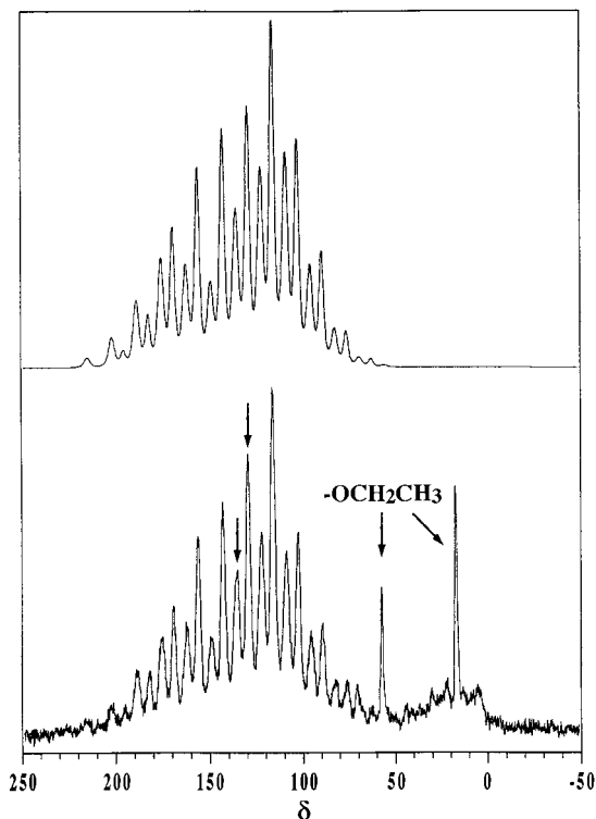
Fig. 10 Low-rotation-speed ^{13}\text{C} CP MAS spectrum (lower) of compound 2 . Only the vinyl CH and \text{CH}_2 patterns are simulated (upper): v_{\text{rot}} = 1000 Hz, \Xi (^{13}\text{C}) = 75.46 MHz, \phi = 7 mm, N_s = 1688 , t_{\text{CP}} = 5 ms, r.d. = 6 s, l.b. = 10 Hz. Isotropic resonances are labelled by arrows
