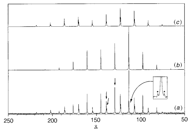
Fig. 3 The ^{13}\text{C} CP MAS NMR spectrum of compound 1 (a), with simulations of CH (b) and \text{CH}_2 (c) patterns. Isotropic resonances are labelled by arrows: \nu_{\text{rot}} = 1200 Hz, \Xi ( ^{13}\text{C} ) = 75.46 MHz, \phi = 7 mm, N_s = 104, t_{\text{CP}} = 5 ms, r.d. = 15 s, l.b. = 3 Hz. * Satellites corresponding to ^1J(^{13}\text{C}-^{29}\text{Si})
