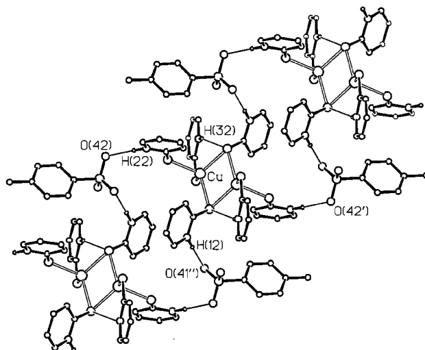
Fig. 4 View of the hydrogen-bonding scheme in complex 3 . The H···O and H···S hydrogen bonds are shown with the thinner lines. The scheme continues in double-linked chains through the crystal
