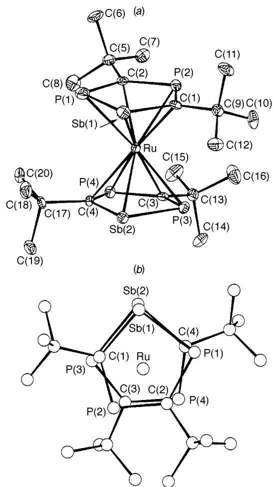
Fig. 2 Molecular structure of the cocrystallised mixture of compounds 20–22 (atomic labels represent 20 )
