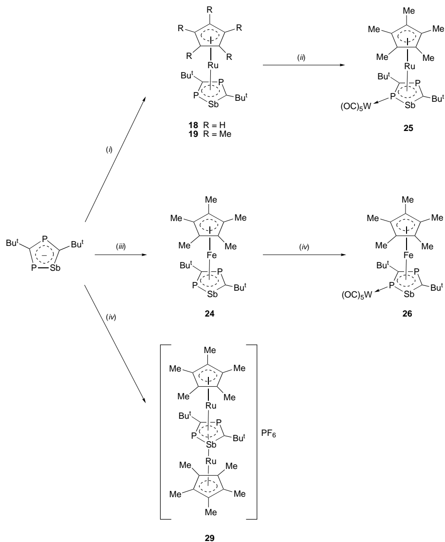
Scheme 2 (i), [\text{Ru}(\text{C}_5\text{R}_5)(\text{MeCN})_3][\text{PF}_6] (R = H or Me), dme, 18 h, 25 °C; (ii) [\text{W}(\text{CO})_5(\text{thf})] , thf, 18 h, 25 °C; (iii) \text{FeCl}_2 , \text{Li}(\text{C}_5\text{Me}_5) , dme, 18 h, 25 °C; (iv) [\text{W}(\text{CO})_5(\text{thf})] , thf, 18 h, 25 °C; (v) 2[\text{Ru}(\text{C}_5\text{Me}_5)(\text{MeCN})_3][\text{PF}_6] , dme, 18 h, 25 °C
