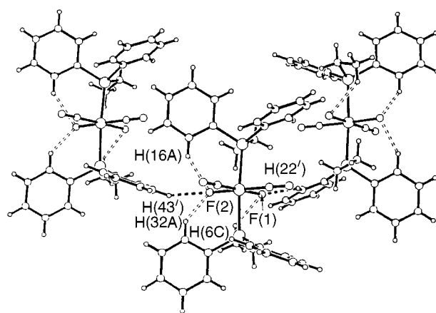
Fig. 4 Extended structure of [OC-6-13][RuF_2(CO)_2(PEtPh_2)_2] showing intermolecular interactions; displacement ellipsoids are shown at the 30% level
