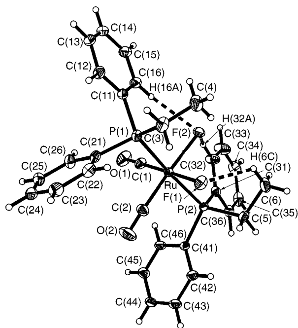
Fig. 3 Molecular structure of [OC-6-13][RuF_2(CO)_2(PEtPh_2)_2] ; displacement ellipsoids are shown at the 30% level
