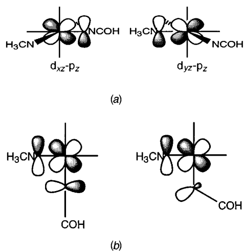
Fig. 7 Formal interpretation of bonding in the crystal structure of complex 3 in the xy plane (a) and in the z direction (b)
