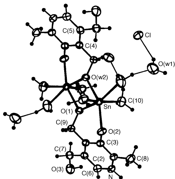
Fig. 4 Crystal structure of [SnMe 2 (H 2 O)(PN-H)]Cl·H 2 O 2 , showing the numbering scheme. Displacement ellipsoids are drawn at the 50% probability level
