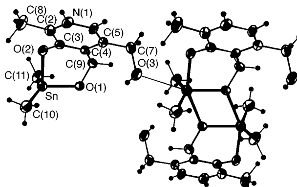
Fig. 1 Crystal structure of [\text{SnMe}_2(\text{PN} - \text{H})\text{NO}_3 \cdot 2\text{H}_2\text{O} 1 , showing the numbering scheme ( \text{NO}_3^- and \text{H}_2\text{O} have been excluded). Displacement ellipsoids are drawn at the 50% probability level
