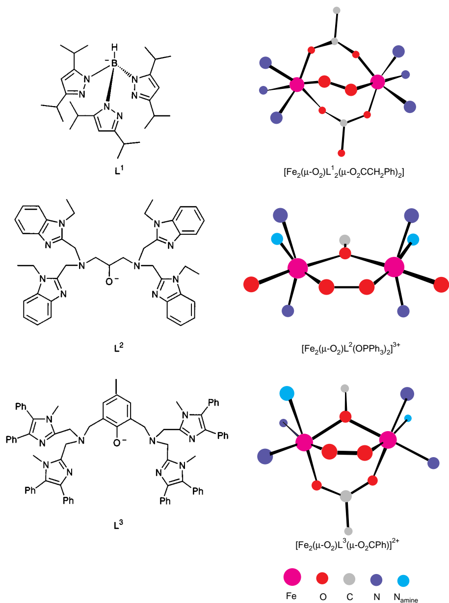
Fig. 2 Structures of synthetic dioxygen adducts from refs. 20–22
