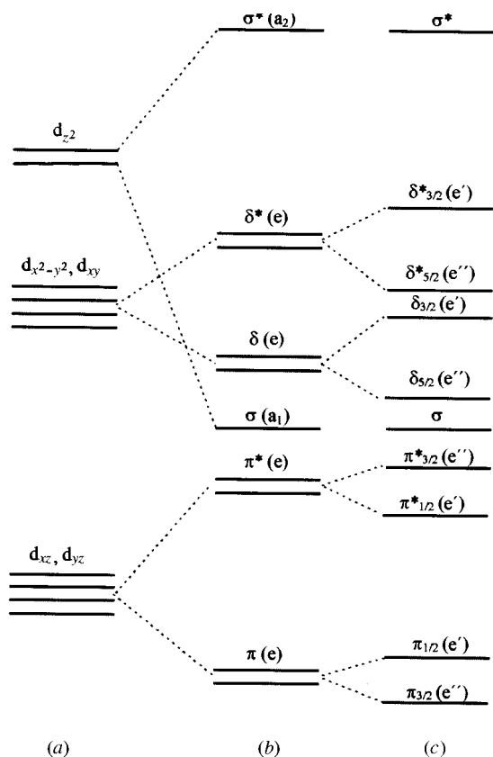
Fig. 2 Proposed energy level diagram of [\text{Cu}_2\text{L}^{\text{imBT}}]^{3+} (a) under C_{3v} , (b) under D_3 and (c) after taking account of the effect of first-order SOC. In (b) the orbitals are labelled according to the angular momentum along the Z axis and according to the representation under D_3 . In (c) the orbitals which transform as e are additionally labelled according to the double group representation. The ordering in (b) has been confirmed by extended Hückel molecular orbital (EHMO) calculations on a simple \text{H}_3\text{N}-\text{Cu}-(\text{NH}=\text{CHCH}=\text{NH})_3-\text{Cu}-\text{NH}_3 model
