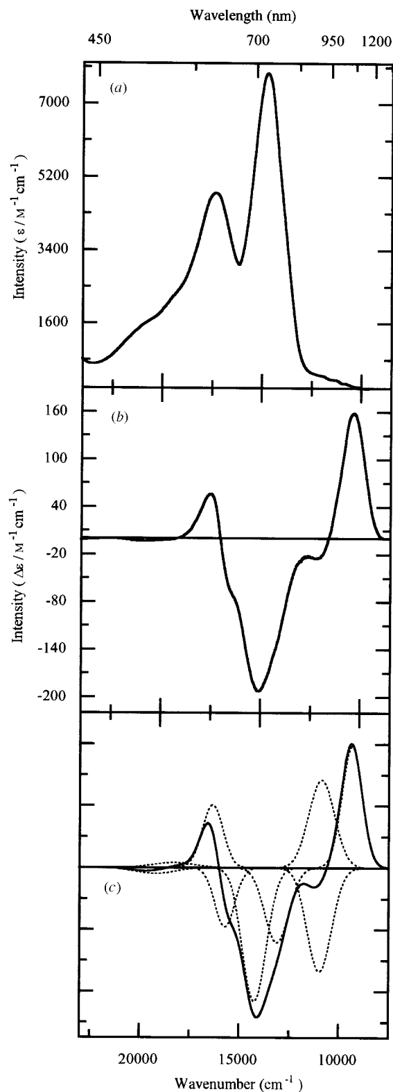
Fig. 3 (a) The 4.2 K absorption spectrum of [\text{Cu}_2\text{L}^{\text{imBT}}]^{3+} obtained in a 1 : 1 (v/v) \text{D}_2\text{O} –ethane-1,2-diol solvent. (b) The 4.2 K MCD spectrum of [\text{Cu}_2\text{L}^{\text{imBT}}]^{3+} obtained in a 1 : 1 (v/v) \text{D}_2\text{O} –ethane-1,2-diol solvent, (c) simulation of the experimental MCD data obtained as the sum of nine Gaussian curves (shown as dotted lines)
