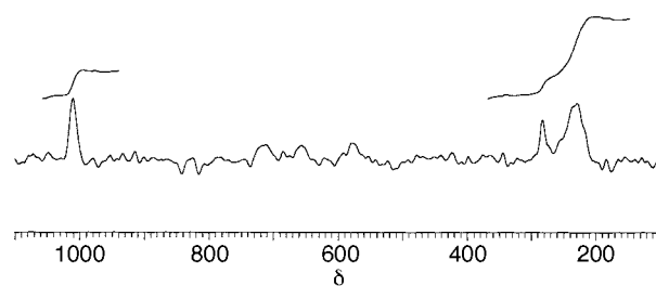
Fig. 8 The ^{17}\text{O} NMR spectrum in D 2 O at pH 9.8, 0.5 \text{ mol dm}^{-3} in V. The main complex ion present is [V(HL)]^{2-} , with resonances assigned in the text
