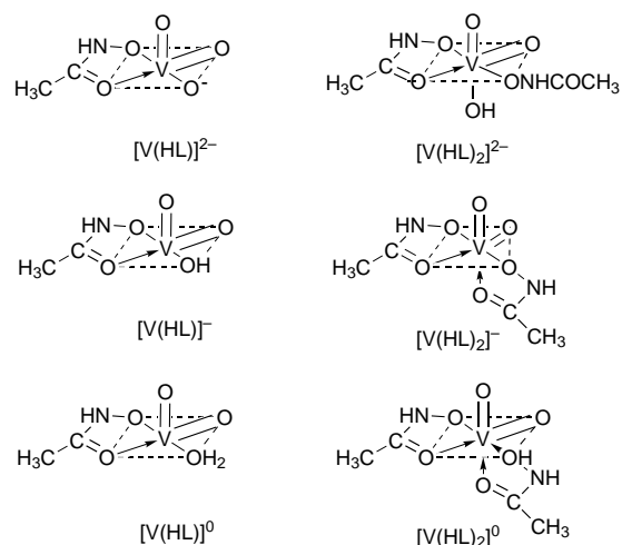
Scheme 1 Tentative structures for the monomeric species, based on shift and linewidth data
