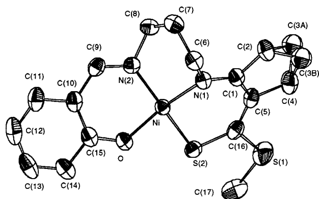
Fig. 1 Molecular structure and crystallographic numbering scheme for [Ni(cdsalpd)]
