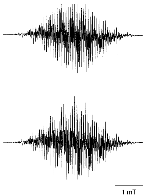
Fig. 2 Experimental (top, THF, 295 K) and simulated (bottom) EPR spectra of [\text{Cr}(\text{CO})_4(\text{bpy})]^{-} enriched with ^{13}\text{C} to 79% (line width 0.013 mT; see text for further information)
