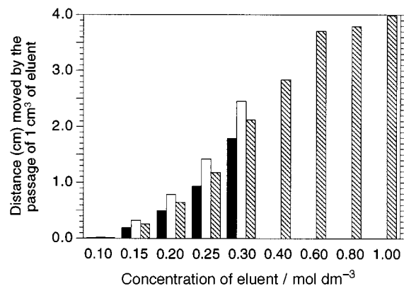
Fig. 5 Relative rate of travel of the diastereoisomers of [\{\text{Ru}(\text{dmbpy})_2\}_2(\mu\text{-bipym})]^{4+} down a 9 mm (inside diameter) column as a function of eluent concentration (aqueous sodium toluene-4-sulfonate) at 30^\circ\text{C} : rac (filled), meso (blank), combined forms (hatched)
