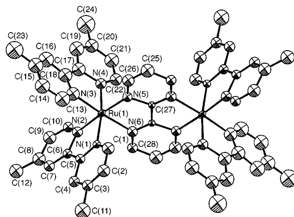
Fig. 3 Thermal ellipsoid plot of meso -(ΛΛ)- \{[Ru(dmbpy)_2]_2(\mu\text{-bipym})\}^{4+} , with ellipsoids drawn at 50% probability. All carbon atoms are isotropic and protons are omitted for clarity
