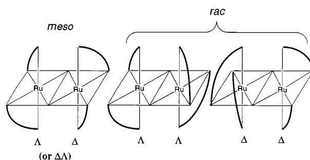
Fig. 1 Schematic view of the isomeric possibilities for the general dinuclear species [\{\text{M}(\text{pp})_2\}_2(\mu\text{-L}_b)]^{n+}
