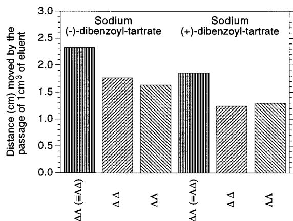
Fig. 8 Relative rate of travel of the three stereoisomers of [\{\text{Ru}(\text{dmbpy})_2\}_2(\mu\text{-bipym})]^{4+} down a 9 mm (inside diameter) column, eluted with aqueous 0.154 \text{ mol dm}^{-3} sodium (+ or -)-dibenzoyltartrate solutions at 30^\circ\text{C}
