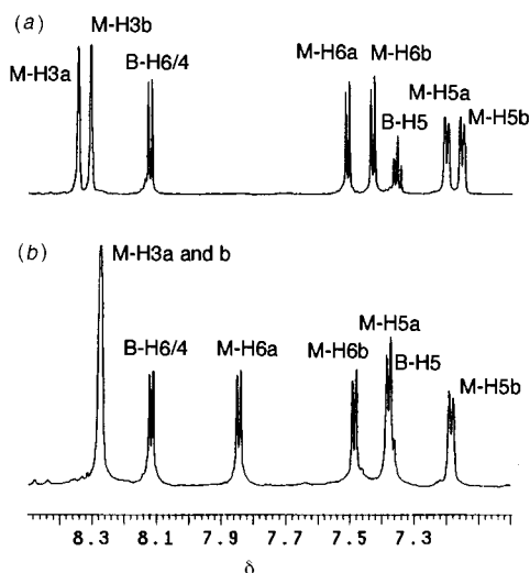
Fig. 2 Proton NMR spectra (500 MHz, 25 °C, D 2 O) of (a) ΔΔ/ΛΛ- and (b) ΔΛ- \{[Ru(dmbpy)_2]_2(\mu\text{-bipym})\}Cl_4
