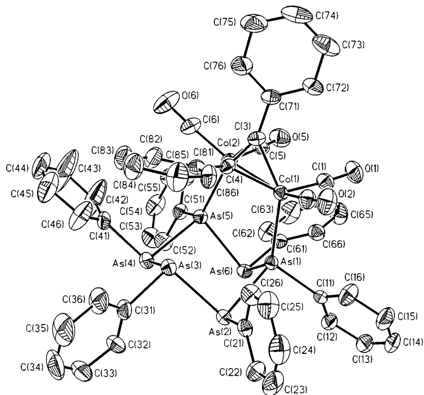
Fig. 4 Molecular structure of [\text{Co}_2(\mu\text{-PhC}\equiv\text{CPh})\{\mu\text{-cyclo}(\text{-PhAs})_6\}(\text{CO})_4] 4 . Details as in Fig. 1
