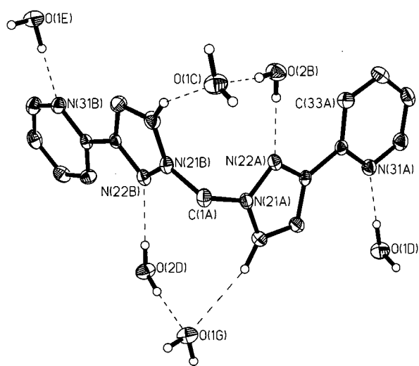
Fig. 1 Structure of L \cdot 4H 2 O, showing the hydrogen-bonding environment around each ligand molecule. Thermal ellipsoids are at the 40% probability level
