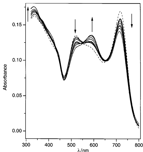
Fig. 6 Spectroscopic titration of [\text{Mn}(\text{oespz})(\text{SH})] (---) with 1-mim in benzene at 20 \pm 0.1 °C. [\text{Mn}]_{\text{tot}} = 0.76 \times 10^{-5} M, [1\text{-mim}] = 0\text{--}0.17 M
