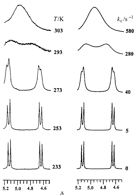
Fig. 2 Variable temperature 1 H NMR spectra of the methylene region (left) for the compound [LCu(PPh 2 CH 2 CH 2 PPh 2 )CuL][ClO 4 ] 2 5 and the corresponding computer simulations (right) in CD 2 Cl 2 solvent.
