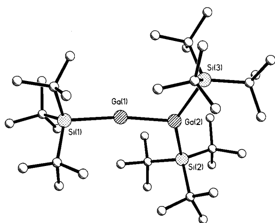
Fig. 4 Schematic drawing of [(\text{Bu}^t_3\text{Si})\text{GaGa}(\text{SiBu}^t)_2] (ref. 63)
