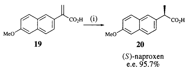
Scheme 5 (i) [\text{Ru}(\text{C}_6\text{H}_6)(\text{BINAP-4SO}_3\text{Na})\text{Cl}]\text{Cl} on CPG-240, ethyl acetate, 95 atm, H 2 , 3 °C.
