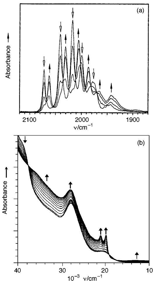
Fig. 4 Spectral changes in the IR \nu(\text{CO}) [(a), in THF at T = 298 \text{ K} ] and UV/VIS [(b), in \text{CH}_2\text{Cl}_2 at T = 253 \text{ K} ] regions, accompanying the reversible reduction of the cluster 1 producing the radical anion 1b
