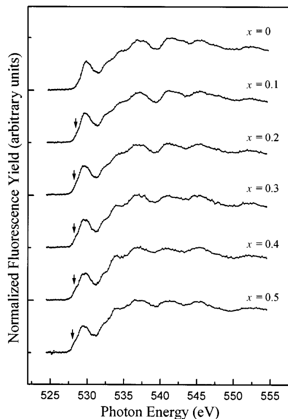
Fig. 2 Oxygen K-edge X-ray absorption near-edge structure spectra for the series of (\text{Cd}_{0.5}\text{Pb}_{0.5})\text{Sr}_2(\text{Ca}_x\text{Y}_{1-x})\text{Cu}_2\text{O}_7 samples in the energy range 525 – 555 eV obtained by the bulk-sensitive total X-ray fluorescence yield technique
