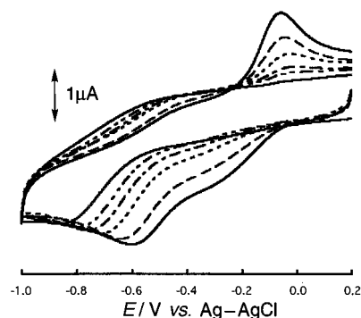
Fig. 7 Cyclic voltammograms of [Co(4-mpyt) 4 PtCl] 2a in 0.1 mol dm -3 Bu 4 NPF 6 -CH 3 CN at a glassy-carbon electrode with a scan rate of 50 mV s -1 at 25 (—), 15 (---), 4 (---), -5 (— · —), -12 (— · — · —) and -25 °C (— · — · —).
