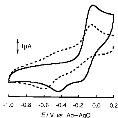
Fig. 5 Cyclic voltammograms of [(CH 3 CN)Co(4-mpyt) 4 Pt] 1 (—) and [Co(4-mpyt) 4 PtCl] 2a (---) in 0.1 mol dm -3 Bu 4 NPF 6 -CH 3 CN at a glassy-carbon electrode with a scan rate of 50 mV s -1 .
