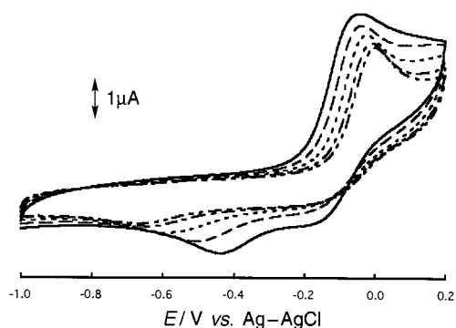
Fig. 6 Cyclic voltammograms of [(CH 3 CN)Co(4-mpyt) 4 Pt] 1 in 0.1 mol dm -3 Bu 4 NPF 6 -CH 3 CN at a glassy-carbon electrode with a scan rate of 50 mV s -1 at 25 (—), 5 (---), -6 (---), -17 (— · —) and -26 °C (— · — · —).
