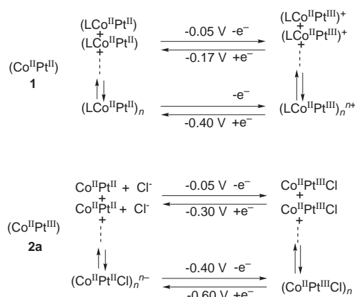
Scheme 2 Square electrochemical-chemical-electrochemical-chemical step dimerization mechanism.
