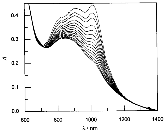
Fig. 1 Decrease of the 1016 nm peak of a DMF solution of \text{CoCp}_2 \cdot \text{C}_{60}(\text{CN})_2 \cdot \text{CS}_2 .
