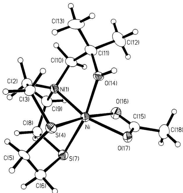
Fig. 4 View of structure of the cation [\text{Ni}(\text{HL}^1)(\text{CH}_3\text{CO}_2)]\text{BPh}_4 \cdot \text{CH}_3\text{CN} with numbering scheme adopted.
