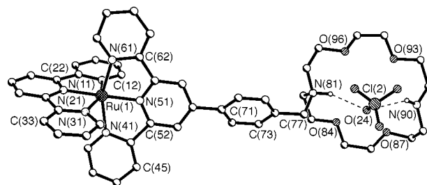
Fig. 1 Crystal structure of the cation [\text{Ru}(\text{tpy})(\text{HL}^1)]^{4+} [\text{ClO}_4]_2 [\text{PF}_6]_2 \cdot 2\text{MeCN} \cdot \text{Et}_2\text{O} \cdot \text{H}_2\text{O} and the hydrogen-bonded perchlorate anion.
