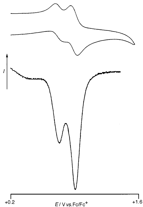
Fig. 3 Cyclic and square-wave voltammograms of [\{(\text{tpy})\text{Ru}(\text{L}^2)_2\}\text{Fe}][\text{PF}_6]_6 in MeCN, showing the \text{Fe}^{\text{II}}\text{--Fe}^{\text{III}} and the two coincident \text{Ru}^{\text{II}}\text{--Ru}^{\text{III}} couples.
