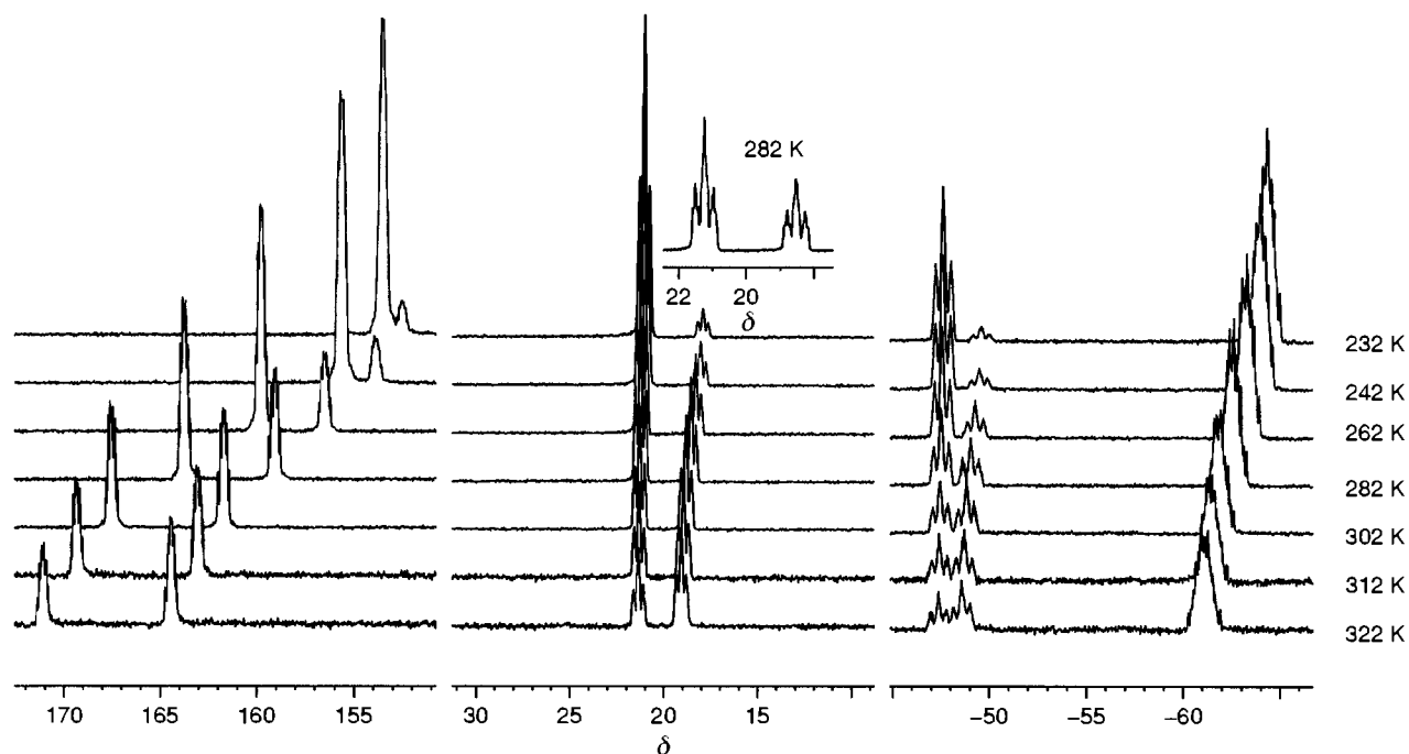
Fig. 4 Variable temperature ^{19}\text{F} NMR spectra of calcium fluoride complex 2 in \text{CDCl}_3 .
