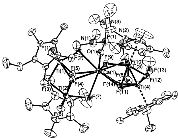
Fig. 1 An ORTEP-like drawing of the adduct [\{Ti_2(C_5Me_4Et)_2F_7\}_2(hmpa)Ca] 4 . Hydrogen atoms are not shown.
