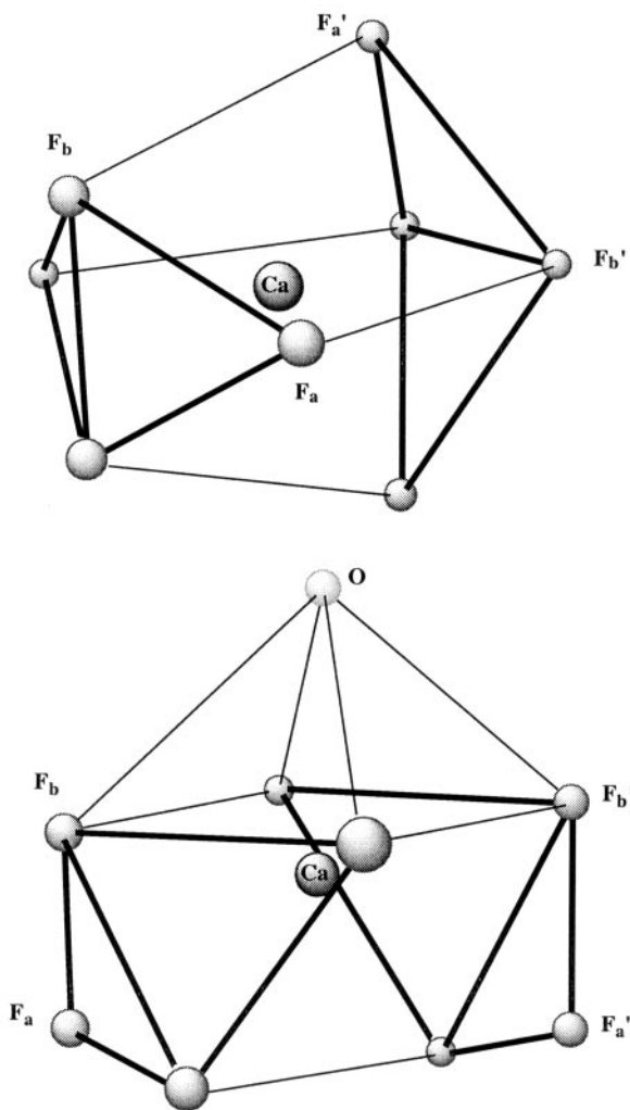
Fig. 2 The dodecahedral (a) (top) and approximate tricapped trigonal prism co-ordination geometry (b) (bottom) of complexes 2 and 4 , respectively. The co-ordinating fluorine atoms ( F_a and F_b ) of each [\text{Ti}_2(\text{C}_5\text{Me}_4\text{Et})_2\text{F}_7]^- moiety are connected by bold lines.
