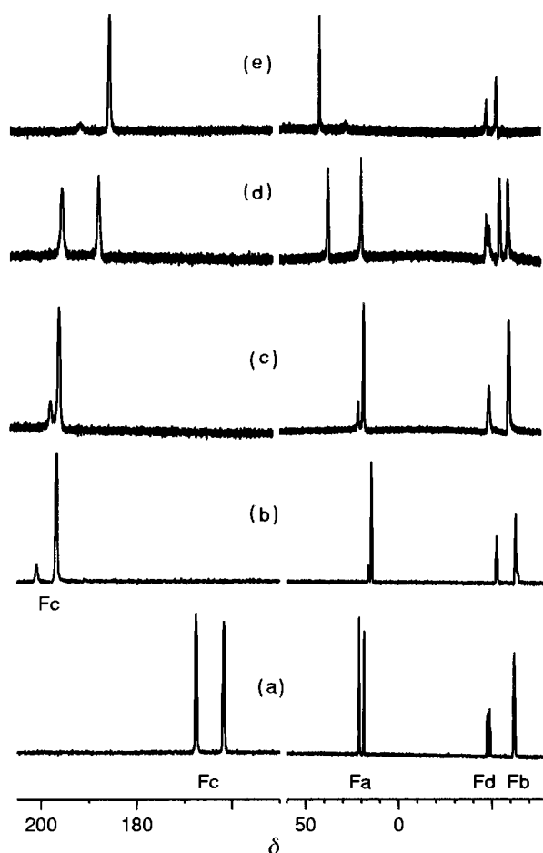
Fig. 3 The ^{19}\text{F} NMR spectra of calcium fluoride complex 2 in (a) \text{CDCl}_3 , (b) [\text{C}_6\text{D}_6][\text{H}_8]\text{thf} , (c) \text{C}_6\text{D}_6 , (d) \text{C}_6\text{D}_6-[\text{C}_6\text{D}_6][\text{H}_8]\text{thf} (20:1) and (e) \text{C}_6\text{D}_6-[\text{C}_6\text{D}_6][\text{H}_8]\text{thf} (2:1). See Scheme 1 for labels.
