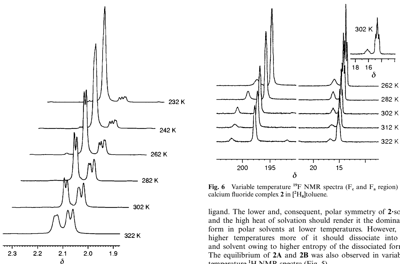
Fig. 5 Variable temperature ^1\text{H} NMR spectra ( \text{C}_5\text{Me}_4\text{Et} resonances) of calcium fluoride complex 2 in \text{CDCl}_3 .
