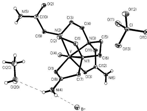
Fig. 2 Molecular structure of [V(O)L]Br[ClO_4] \cdot MeOH 2 .
