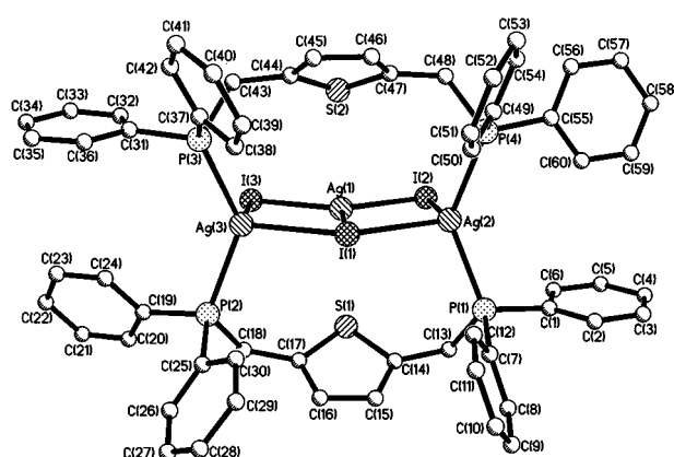
Fig. 2 Perspective view of the structure of [Ag 3 ( \mu_3 -I)( \mu -I) 2 ( \mu -dpmt) 2 ] 4 with atomic numbering scheme.
