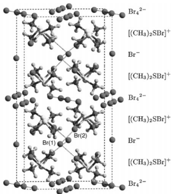
Fig. 3 A view of the structure of the orthorhombic phase (\text{CH}_3)_2\text{SBr}_{2.5} . The nature of the ionic layers is indicated at the right. Atoms are shaded as in Fig. 2, and Br(1) and Br(2) are indicated. See Fig. 5a for the labelling of the other bromine atoms.
