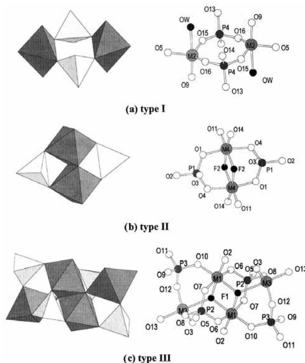
Fig. 1 Secondary building units: (a) type I [ \text{Al}_2\text{P}_2\text{O}(\text{H}_2\text{O})_2 ]; (b) type II ( \text{Al}_2\text{P}_2\text{O}_7 ); (c) type III ( \text{Al}_4\text{P}_4\text{O}_7 ).
