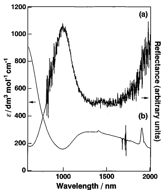
Fig. 1 (a) Reflectance spectrum of [\text{Fe}_2(\text{bpmp})(\text{ppa})_2][\text{BF}_4]_2 3 appropriately diluted with \text{BaSO}_4 . (b) Absorption spectrum ( 1 \times 10^{-3}\text{ mol l}^{-1} ) in acetonitrile.
