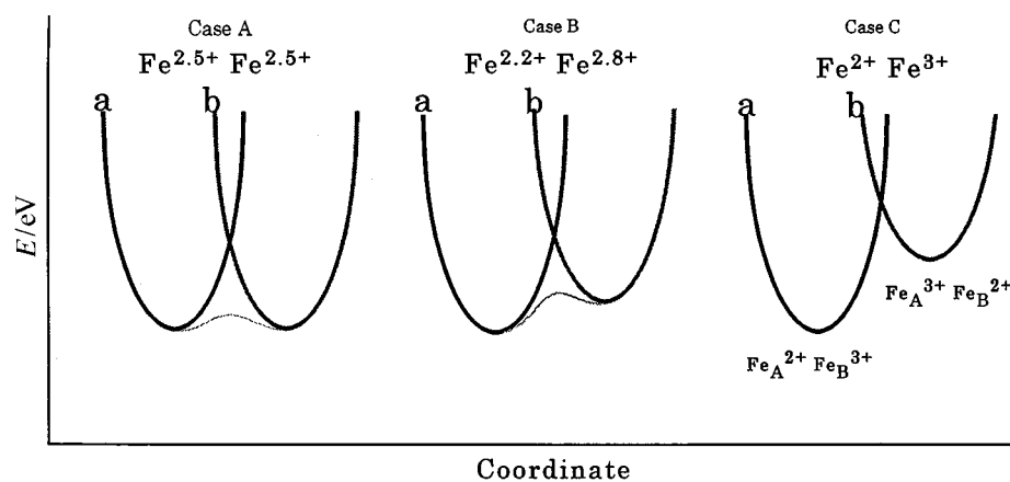
Fig. 9 Potential energy diagrams for mixed-valence dinuclear iron(II,III) complexes. Curve a is for the \text{Fe}_A^{2+}\text{Fe}_B^{3+} state and b for \text{Fe}_A^{3+}\text{Fe}_B^{2+} . Case A: for delocalized valence states. Case B: for energetically inequivalent vibronic states. An excess electron (a valence electron of \text{Fe}^{2+} ) stays 80% of the time in the \text{Fe}_A^{2+}\text{Fe}_B^{3+} state and 20% in the \text{Fe}_A^{3+}\text{Fe}_B^{2+} state. Case C: for localised valence states.
