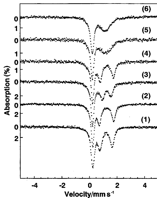
Fig. 2 Mössbauer spectra for the complexes 1–6 at 298 K.
