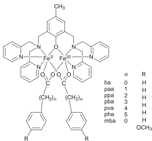
Chart 1 [\text{Fe}_2(\text{bpmp})(\text{L})_2]^{2+} .
