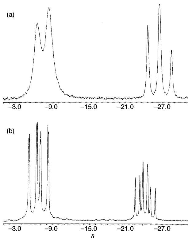
Fig. 1 ^{31}\text{P}\text{-}\{^1\text{H}\} NMR spectra of [\text{Ag}(\text{TP})\text{Cl}] in \text{CD}_2\text{Cl}_2 at 20 (a) and -70^\circ\text{C} (b).
