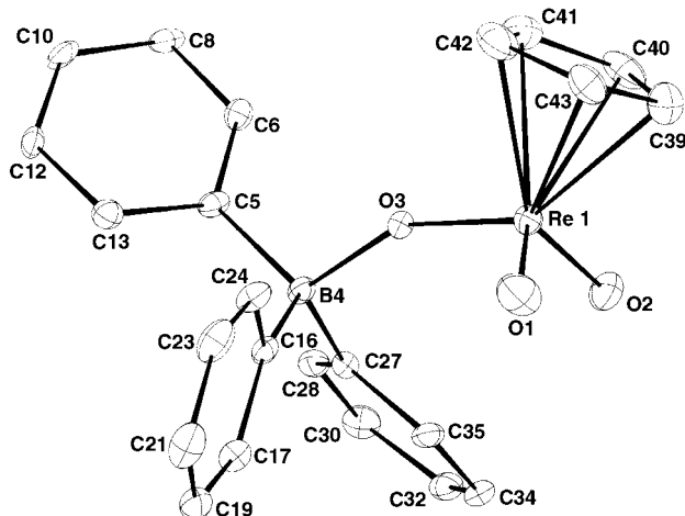
Fig. 2 Crystal structure of 6 , [\text{Re}(\eta\text{-C}_5\text{H}_5)\text{O}_2\{\text{OB}(\text{C}_6\text{F}_5)_3\}]_2 , with fluorine atoms removed for clarity.
