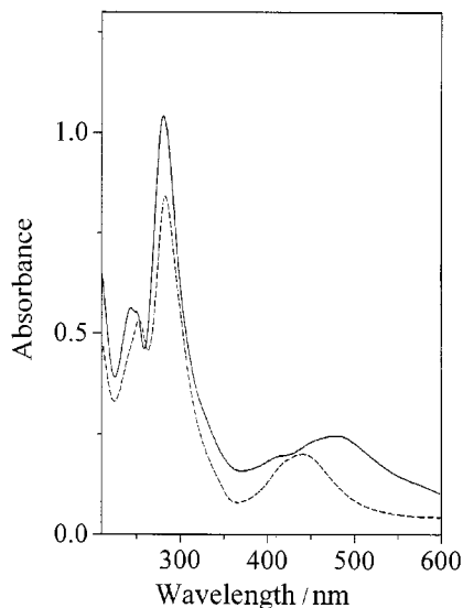
Fig. 4 Absorption spectra of the mononuclear complex 1 (---) and of binuclear complex 2 (—) in water at the same concentration of 10 \mu\text{mol dm}^{-3} .
