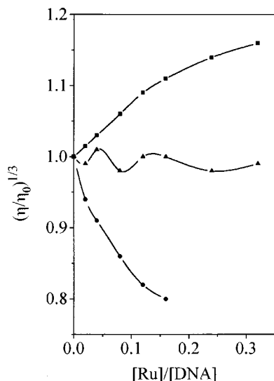
Fig. 6 Effect of increasing amounts of [\text{Ru}(\text{bpy})_3]^{2+} (▲), [\text{Ru}(\text{bpy})_2(\text{pztp})]^{2+} (■) and [(\text{bpy})_2\text{Ru}(\text{pztp})\text{Ru}(\text{bpy})_2]^{4+} (●) on the relative viscosities of calf thymus DNA at 32.7 \pm 0.1 °C.
