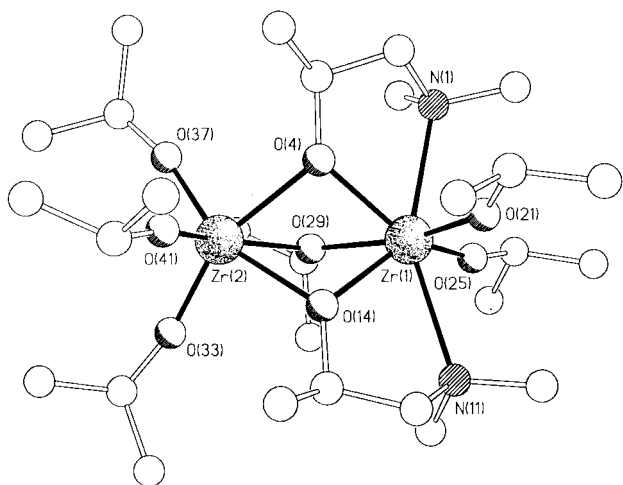
Fig. 1 Molecular structure of [Zr 2 (OPr i ) 6 (dmap) 2 ] 3 .
