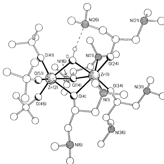
Fig. 3 Molecular structure of [\text{Zr}_2(\text{OBu}^t)_3(\text{bdmap})_4(\text{OH})] 5 .
