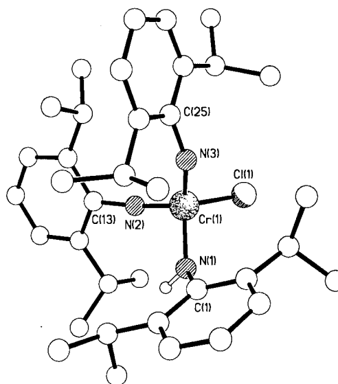
Fig. 2 The molecular structure of compound 3 .
