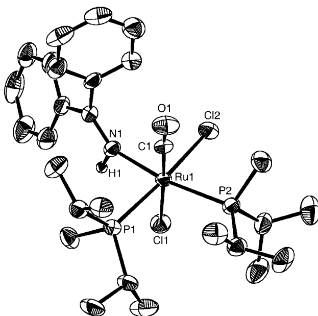
Fig. 1 An ORTEP 15 drawing of the compound [\text{RuCl}_2(\text{CO})(\text{NH}=\text{CPh}_2)(\text{P}^i\text{Pr}_2\text{Me})_2] 4 .
