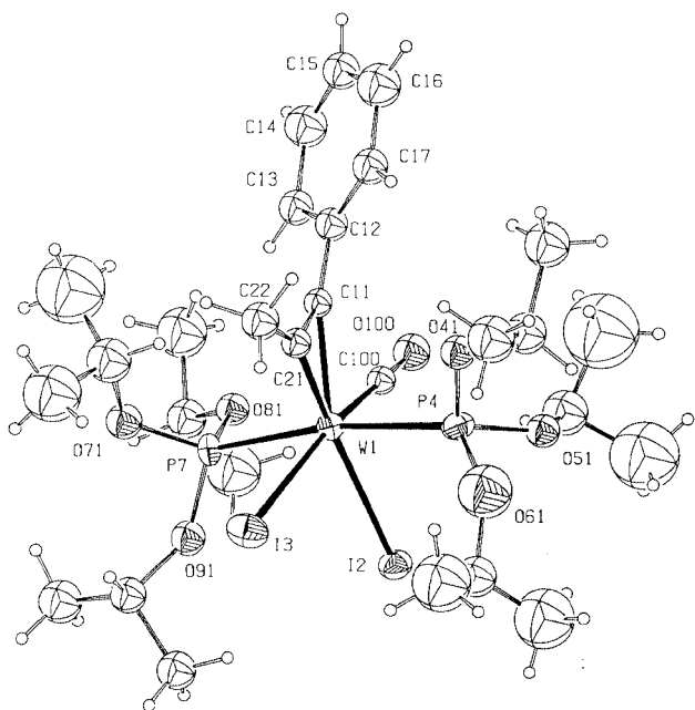
Fig. 8 An ORTEP diagram showing the structure of trans -[W 12 (CO) 3 {P(O i Pr) 3 } 2 (η 2 -MeC 2 Ph)] 16 and the atom numbering scheme.
