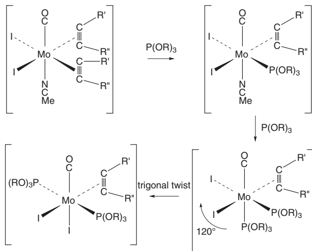
Scheme 1 Proposed mechanism for the stepwise reaction of two equivalents of P(OR) 3 with [MoI 2 (CO)(NCMe)(η 2 -R' 2 C 2 R'')] \{R = \text{Ph}, R' = \text{Me}, R'' = \text{Ph}\} .
