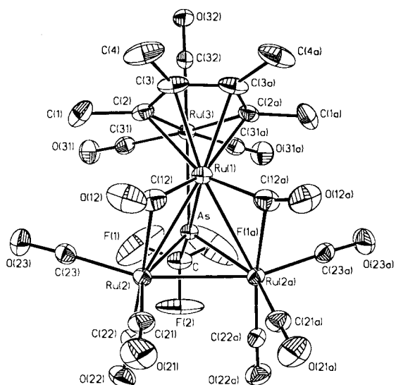
Fig. 6 Molecular structure of compound 9 . Important bond lengths and angles which do not appear in the text: Ru(1)–Ru(2) 2.870(1), Ru(1)–Ru(3) 2.797(1), Ru(2)–Ru(2a) 2.780(1), Ru(1)–As 2.579(1), Ru(2)–As 2.422(1), Ru(3)–As 2.595(1), Ru(1)–C(2) 2.225(6), Ru(1)–C(3) 2.268(6), Ru(3)–C(2) 2.123(6), C(2)–C(3) 1.406(8) and C(3)–C(3a) 1.449(15) Å; Ru(2)–Ru(1)–Ru(3) 101.7(1), Ru(2)–Ru(1)–Ru(2a) 57.9(1), Ru(1)–Ru(2)–Ru(2a) 61.0(1), Ru(3)–C(2)–C(3) 116.0(4), C(2)–C(3)–C(3a) 114.6(4) and C(2)–Ru(3)–C(2a) 76.1(3)°.
