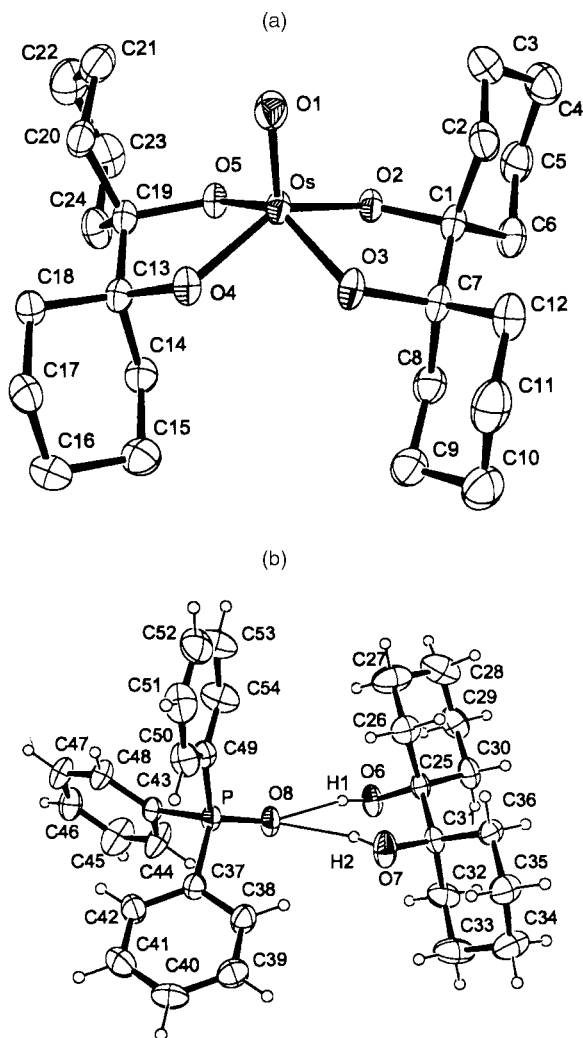
Fig. 2 (a) An ORTEP view of the osmium(vi) unit in complex 2 with 30% thermal ellipsoids showing the atom labelling system of the heavy atoms. (b) An ORTEP view of the triphenylphosphine oxide-diol unit with 30% thermal ellipsoids showing the atom labelling system of the heavy atoms and HO hydrogens.
