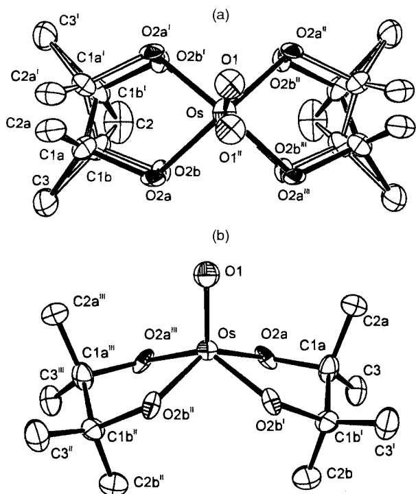
Fig. 1 (a) An ORTEP 18 view of complex 1 in the disordered position with 30% thermal ellipsoids showing the atom labelling scheme. Hydrogen atoms are not included and one half of all atoms and symmetry-related oxygens are labelled. Symmetry operations: I 1 - y, 1 - x, z ; II 1 - x, 1 - y, z ; III y, x, z . (b) An ORTEP view with 30% thermal ellipsoids showing the atom labelling system. Hydrogen atoms are not shown.
