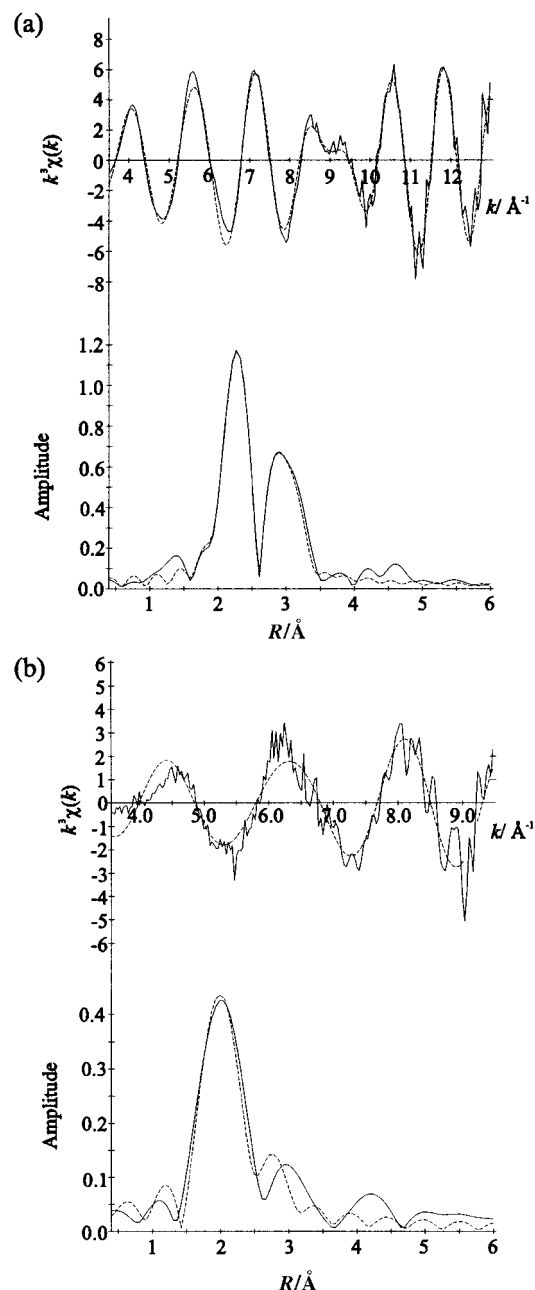
Fig. 2 EXAFS Spectra of [\text{NH}_4]_2[\text{W}_3\text{S}_{16}(\text{NH}_3)_3]^{2-} from (a) the tungsten \text{L}_{\text{III}} -edge and (b) the sulfur K-edge (top k^3 -weighted EXAFS and bottom its Fourier transform; (—) experimental and (---) theoretical).
