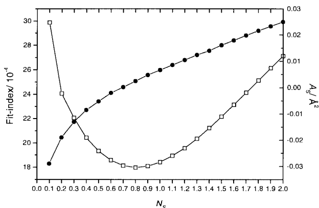
Fig. 4 The effect on sulfur K-edge EXAFS fit index (unfilled squares) and Debye–Waller factor (filled circles) of the occupation number of the sulfur shell at 2.06 Å for [\text{NH}_4]_2[\text{W}_3\text{S}_{16}(\text{NH}_3)_3] .
