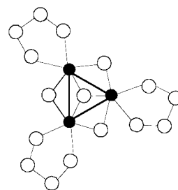
Fig. 3 A sketch of the [\text{W}_3(\mu_3\text{-S})(\mu\text{-S})_3(\text{S}_4)_3(\text{NH}_3)_3]^{2-} anion found in [\text{NH}_4]_2[\text{W}_3\text{S}_{16}(\text{NH}_3)_3] , used as a model compound in the EXAFS experiments. Unfilled circles represent sulfur atoms and filled circles, tungsten. Co-ordinated ammonia molecules (one per tungsten atom) are omitted for clarity.
