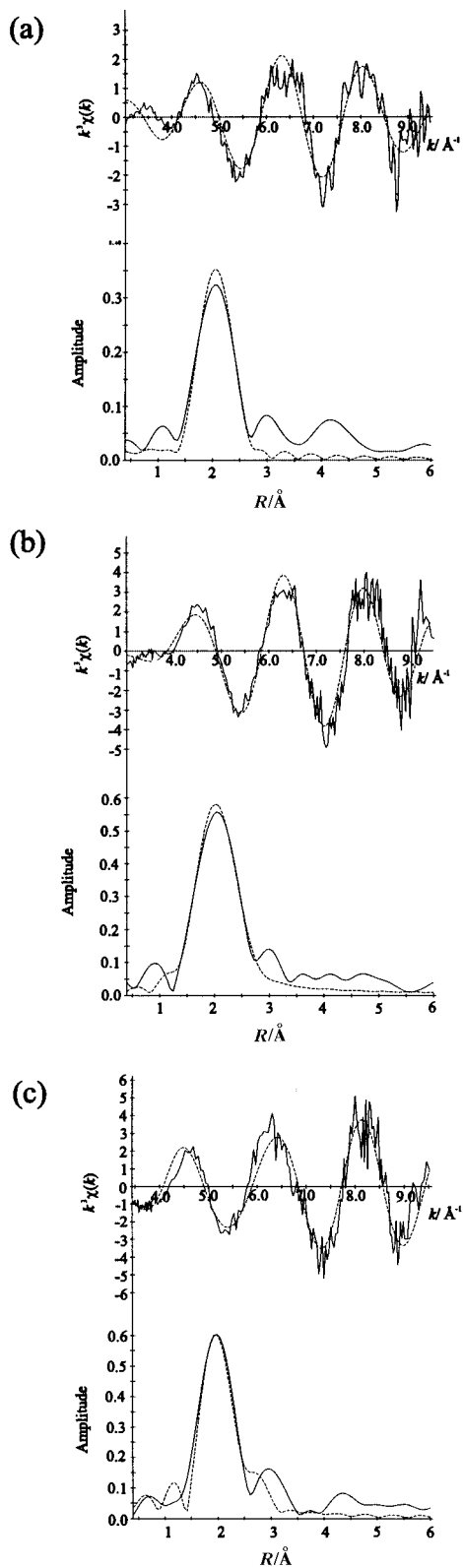
Fig. 5 Sulfur K-edge EXAFS for (a) \text{WS}_3 , (b) \text{WS}_5 and (c) \text{Re}_2\text{S}_7 ; top k^3 -weighted EXAFS (—) experimental and (----) theoretical and bottom the Fourier transform.
