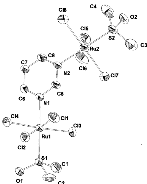
Fig. 4 An ORTEP view of the anion of Na_2[\{trans-RuCl_4(Me_2SO-S)\}_2(\mu-pym)]^- 1b . Details as in Fig. 1.
