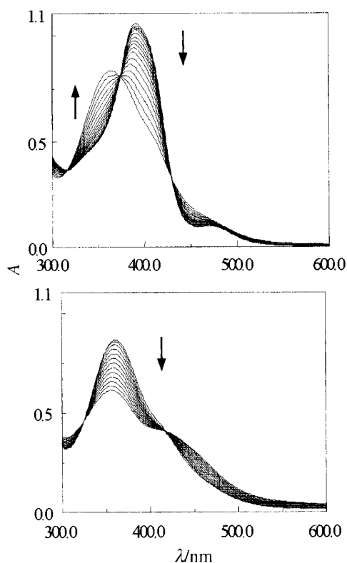
Fig. 5 Spectral changes in the visible region during stepwise chloride hydrolysis from Na 2 [ trans -RuCl 4 (Me 2 SO-S)] 2 ( \mu -pyz)] 1a (25.0 °C, 0.1 mol dm -3 phosphate buffer, pH 7.4, 0.9% NaCl, [1a] = 10 -4 mol dm -3 , scan-time interval = 10 min). Top, first step; bottom, second step.
