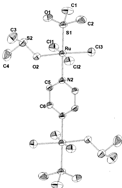
Fig. 3 An ORTEP view of [\{mer,cis-RuCl_3(Me_2SO-S)(Me_2SO-O)\}_2(\mu-pyz)]^- 3a . Details as in Fig. 1.
