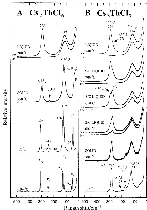
Fig. 1 Raw Raman spectra of: (A) Cs 2 ThCl 6 in the solid and liquid phases; the assignments are based on Table 2 and the correlation diagram O_h \rightarrow D_{3d} given in the text; (B) Cs 3 ThCl 7 in the solid, liquid and supercooled liquid phases; the assignments are based on the refs. in Table 3. Spectral conditions: laser line \lambda_0 = 488.0 nm, laser power, w = 100 mW, spectral slit width (ssw) = 3 cm -1 , scan rate 2 cm -1 s -1 .
