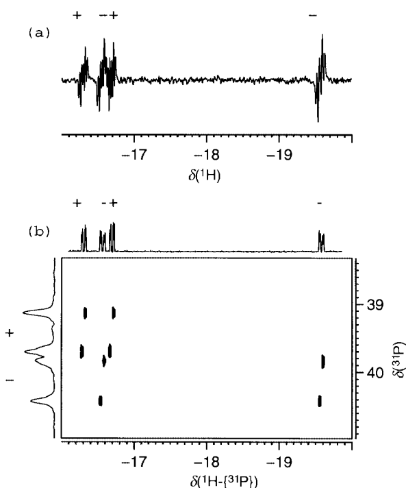
Fig. 2 The NMR spectra of the products 2-[I-I-Ph] and 2-[Cl-I-Ph] formed by warming RhCl(CO)(PPh_3)_2 , 1-[Cl-Ph] , and RhI(CO)(PPh_3)_2 , 1-[I-Ph] , in the ratio 8:1 with p-H_2 in C_6D_6 at 313 K: (a) ^1H spectrum showing the hydride resonances; (b) selected cross peaks (absolute value display) and projections in the ^1H-^{31}P HMQC correlation spectrum showing hydride and phosphorus chemical shift connections ( ^{31}P decoupled).
