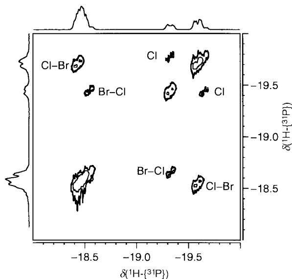
Fig. 8 The 1 H- {31}P EXSY spectrum (absolute value display) of a sample containing complexes 2-[Cl-Cl-Ph], 2-[Br-Br-Ph], 2-[Cl-Br-Ph] and 2-[Br-Cl-Ph], formed by warming 1-[Cl-Ph] and 1-[Br-Ph] with p-H 2 in C 6 D 6 at 316.6 K for a mixing time of 0.1 s. Exchange peaks connecting the hydride resonances of 2-[Cl-Cl-Ph], 2-[Cl-Br-Ph] and 2-[Br-Cl-Ph] are indicated.
