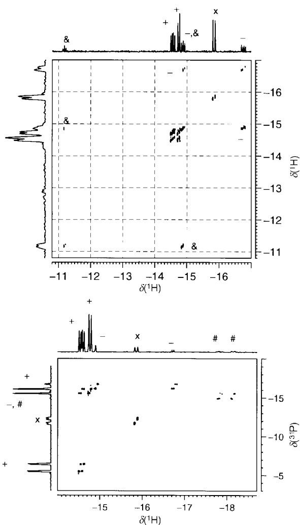
Fig. 5 The 2-D NMR spectra of the products formed by warming RhI(CO)(PMe 3 ) 2 , 1-[I-Me], with p-H 2 in C 6 D 6 at 343 K: (a) selected cross peaks (absolute value display) and projections in the ^1\text{H} - ^1\text{H} COSY spectrum of 3-[I-H-Me](+), 3-[H-I-Me](-), 2-[I-I-Me](#) and 4-[H-I-I-Me](&) (x = RhH 2 Cl(PMe 3 ) 3 , ^{31}\text{P} decoupled); (b) selected cross peaks (absolute value display) and projections in the ^1\text{H} - ^{31}\text{P} HMQC correlation spectrum ( ^{31}\text{P} decoupled), details as in (a).
