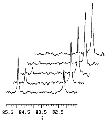
Fig. 1 The ^{31}\text{P}\text{-}\{^1\text{H}\} NMR spectra recorded during the reaction of trans\text{-[FeH(MeCN)(DPPE)}_2\text{]}^+ with 2,6-(MeO) 2 C 6 H 3 CN excess in [D 6 ]acetone solution at 35 °C. The spectra were recorded at 922 s intervals and show the complete conversion into trans\text{-[FeH(2,6-(MeO)}_2\text{C}_6\text{H}_3\text{CN)(DPPE)}_2\text{]}^+ . The concentrations of iron complex and incoming ligand were close to 1 \times 10^{-3} and 0.05 \text{ mol dm}^{-3} , respectively.
