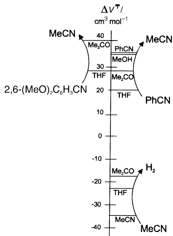
Fig. 2 Graphical presentation of \Delta V^\ddagger values for substitution reactions of trans - [\text{FeH}(\text{L})(\text{DPPE})_2]^+ complexes (L = \text{H}_2 or MeCN). Horizontal lines connected to a common arrow represent the values obtained for the same reaction in different solvents, and the labels at both ends of the arrows indicate the leaving and incoming ligands.
