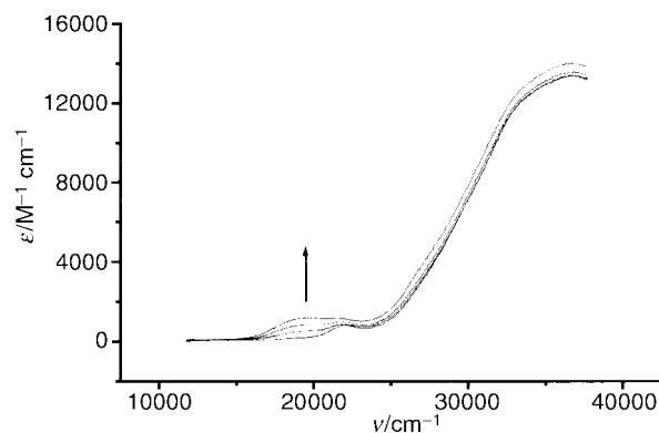
Fig. 2 Electrogeneration of cation 3 2+ followed by uv/vis spectrometry.
